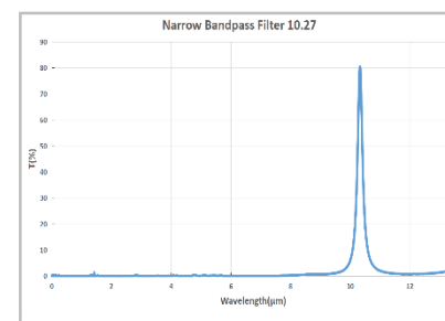
(12) 10.27-200nm narrow band pass filter
